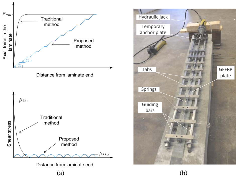
Figure 1. (a) Axial force in the laminate and the corresponding interfacial shear stress in the bond line and (b) The prestressing device and set up during prestressing
